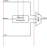
Figure 2.7: RV32ICore WB Stage
