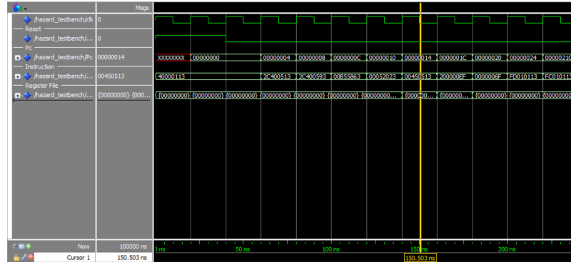
Figure 3.1: RV32ICore Initialization
